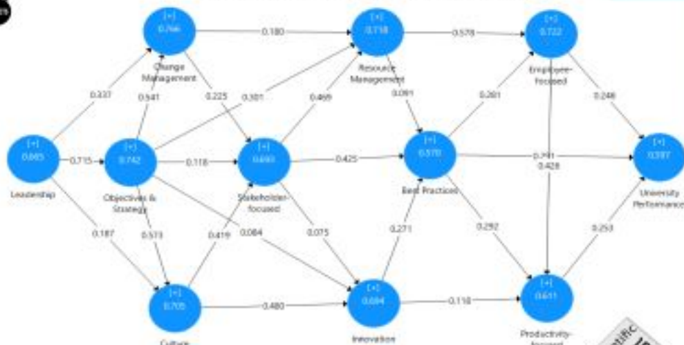
Instrument validation through assessment of measurement model using partial least squares – structural equation modelling
